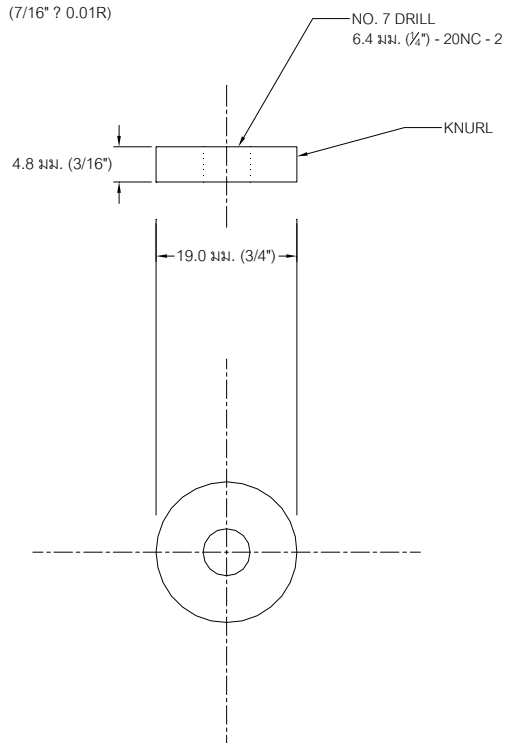
LOWERING SCREW
