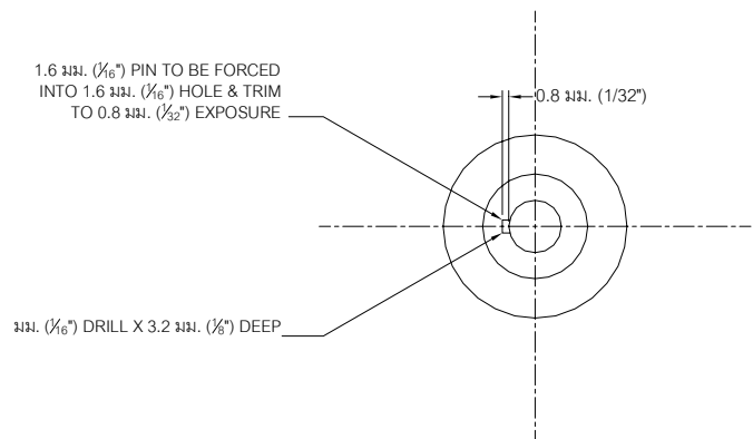
TENSION HEAD
